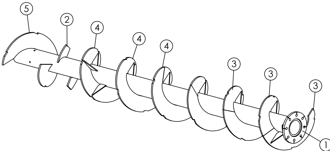
#872720RH - 720-16 RIGHT HAND DISCHARGE EXTRA DUTY BOTTOM AUGER WA
