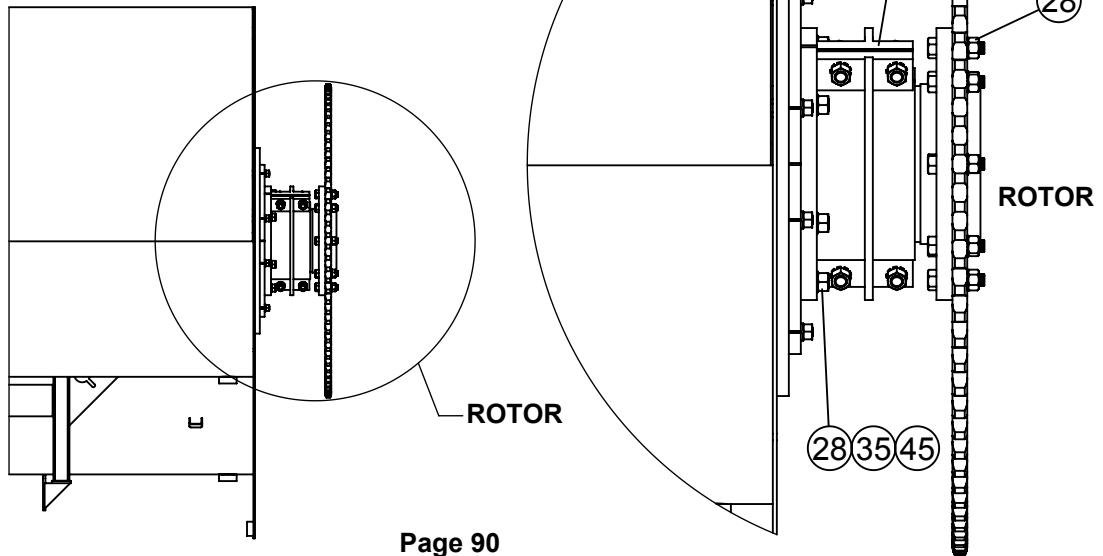
DRIVE ASSEMBLY WITH ONLY THE ROTOR SHOWN
